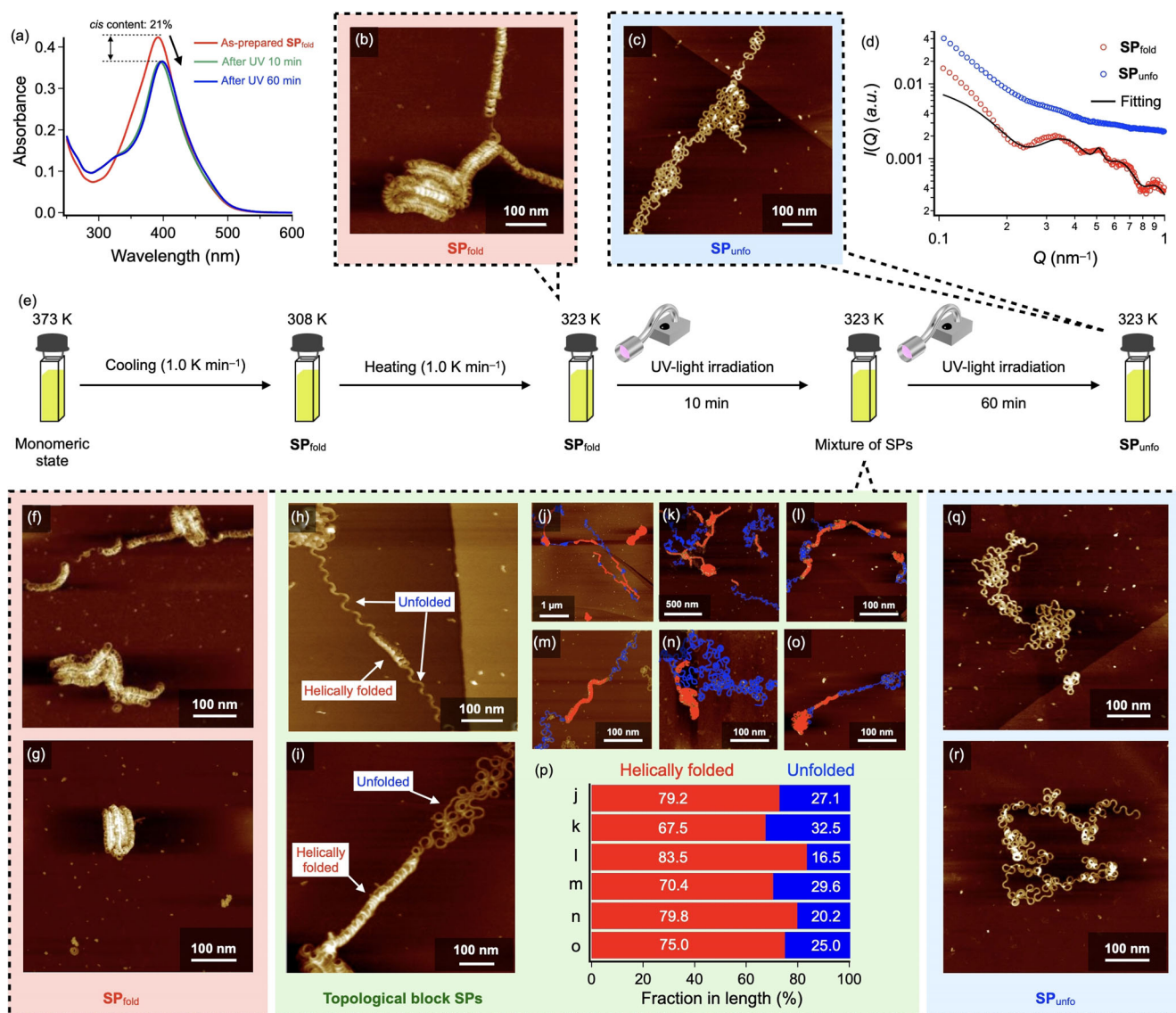
Figure 3. a) UV-Vis spectra of a MCH solution of 2 ( c = 10 \mu\text{M} ) during UV-light irradiation at 323 K. b, c) AFM images of SP_{fold} of 2 before UV-light irradiation (b) and SP_{unfo} of 2 after UV-light irradiation for 60 min at 323 K (c). d) Change of SAXS profiles of a SP_{fold} solution of 2 ( c = 50 \mu\text{M} ) upon UV-light irradiation at 323 K (from red to blue). The black line is a fit to the data using a core-multishell cylinder model. e) Schematic representation of procedure on photo-induced unfolding of SP_{fold} of 2 (f-o, q, r) AFM images of SP_{fold} (f, g), topological block SPs (h-o), and SP_{unfo} (q, r) found in a solution of 2 upon UV-light irradiation for 10 min at 323 K. In (j-o), helically folded and unfolded domains were colored with red and blue, respectively. p) Fractions in length of helically folded and unfolded domains in the topological block SPs.
